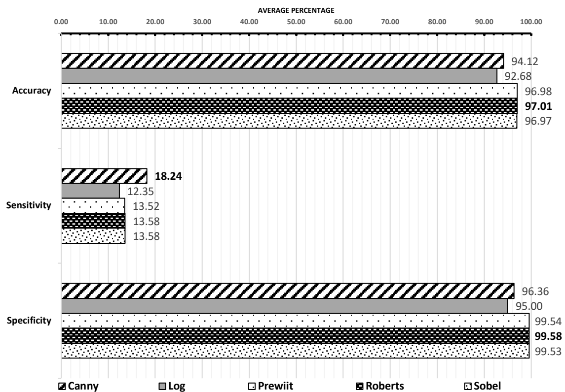
Fig. 10. Average performance comparison of segmentation methods across all samples
