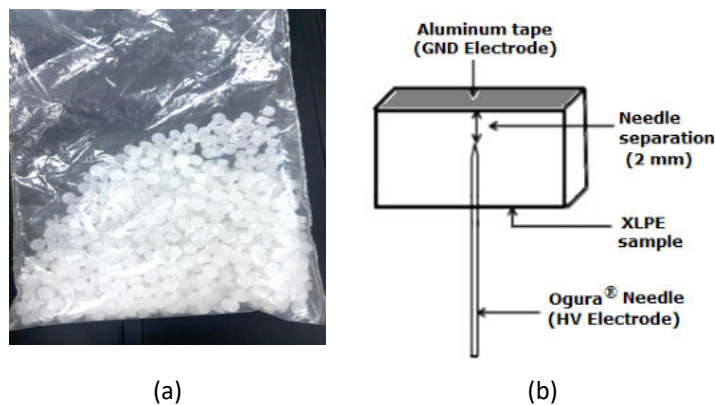
Fig. 2. Sample preparation (a) XLPE beads (b) Planar-to-plane electrode configuration
