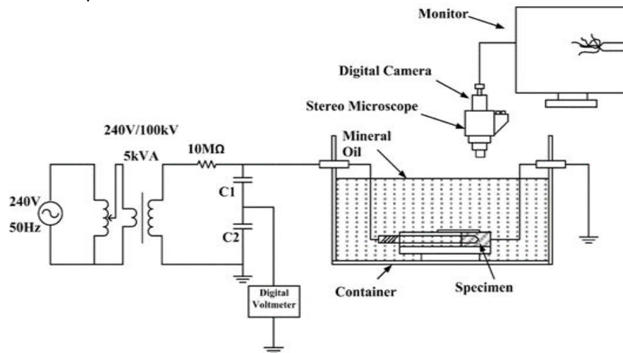
Fig. 3. Electrical tree data acquisition setup
