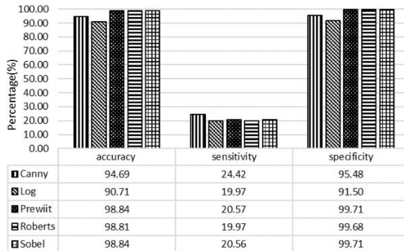
Fig. 8. Performance comparison of segmentation methods for S_4
