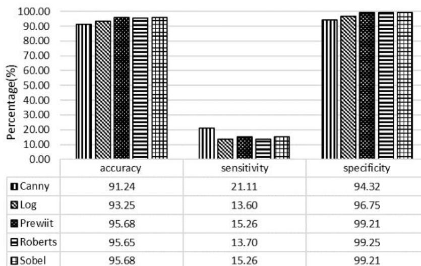
Fig. 7. Performance comparison of segmentation methods for S_3
