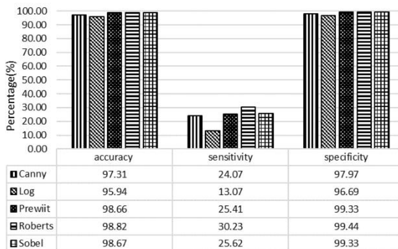
Fig. 9. Performance comparison of segmentation methods for S_5
