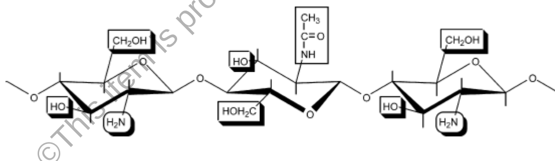
Figure 2.4: Illustration of the possible reaction sites in chitin and chitosan.
