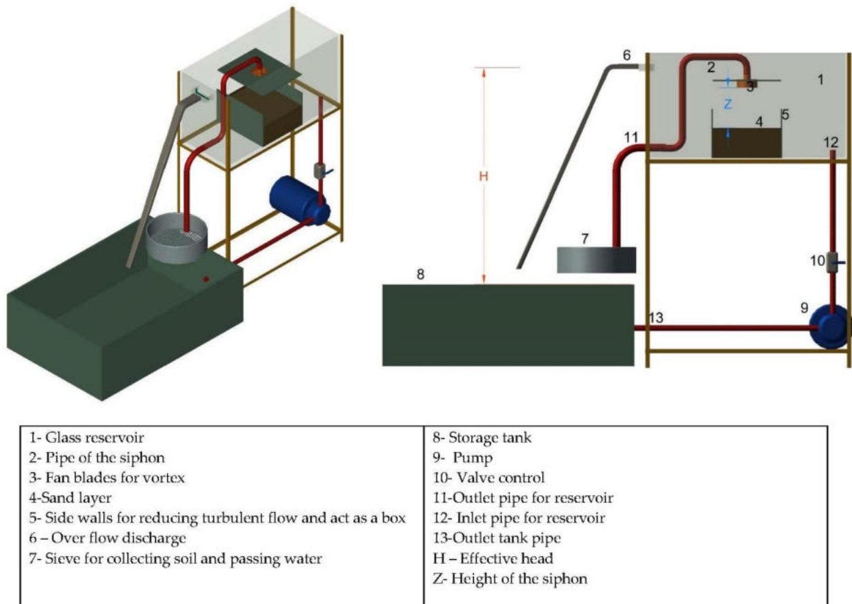
Figure 1. The laboratory tank model and description of parts.
