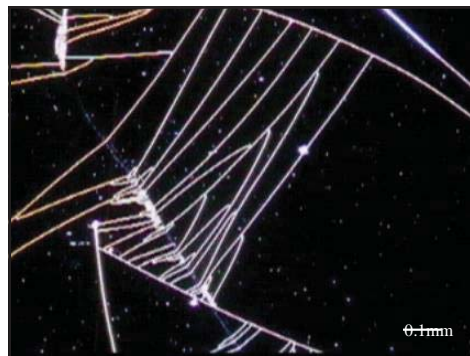
Figure 7(b). Optical microscope dark field image of silica-titania thicker film exhibited crack advancing toward each other forming spider web crack pattern. (5x mag.).
