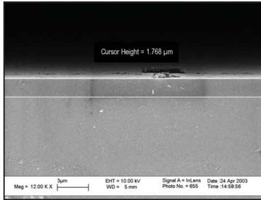
Figure 4. SEM micrograph of silica based crack film with 10 times RTA at 680°C. Further deposition for building up thicker layer was not able to proceed above 1.77μm thickness.
