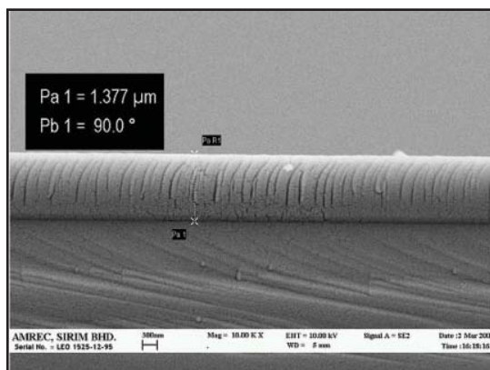
Figure 3. SEM micrograph of crack free thin film silica-titania (prepared from 10% titania + 90% silica sol) at 680°C with thickness of 1.38µm.
