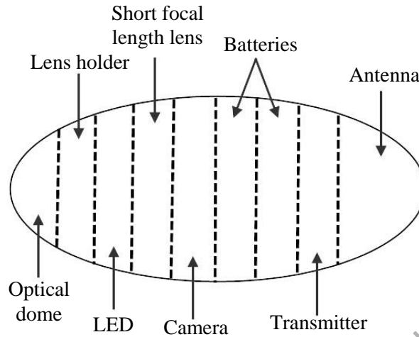
Figure 1.3: Ingestible wireless biomedical device layout.
