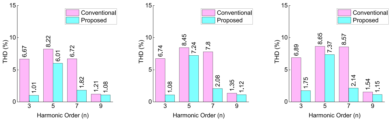
Fig.17 The percentage of low-order harmonic content for inverter ratio 100:50 ratio using conventional and proposed sector definitions (a) high speed (b) medium speed (c) low speed.
