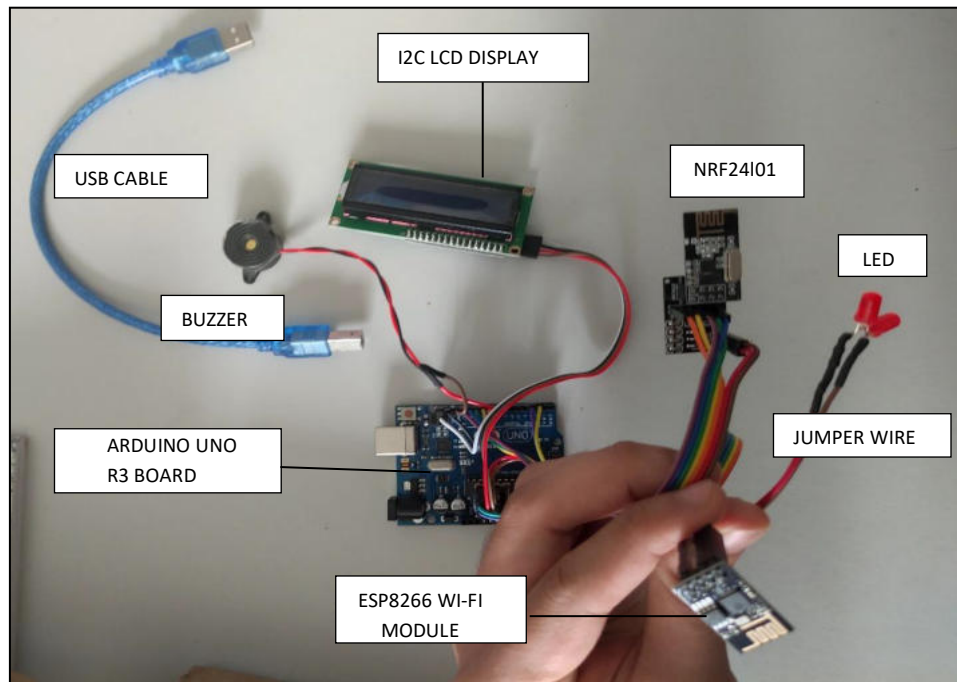
Fig. 4. The circuit installation of the proposed earthquake detection system (a) Transmitter part, (b) Receiver part
