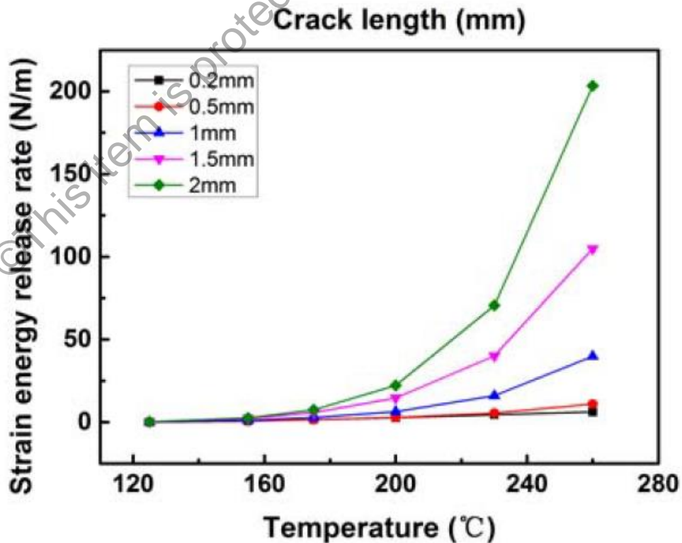
Figure 2.4 Effect of temperature on strain energy release rate. Source: Wang (2016)
