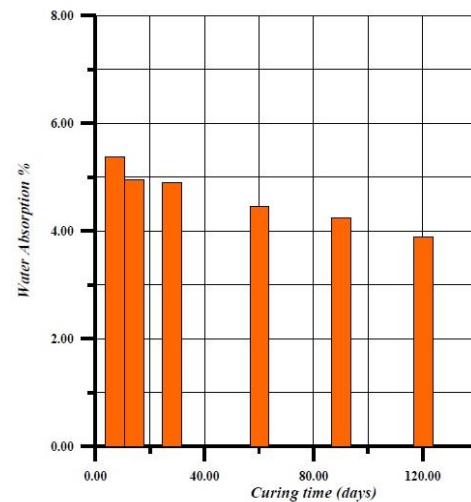
Figure 9. Water absorption for (20% CBM)
