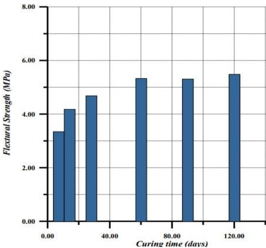
Figure 22. Flexural strength for 10% (DBM)
