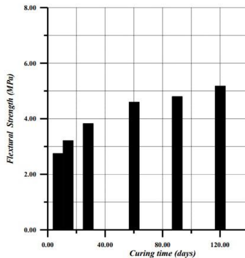
Figure 19. Flexural strength for reference specimens
