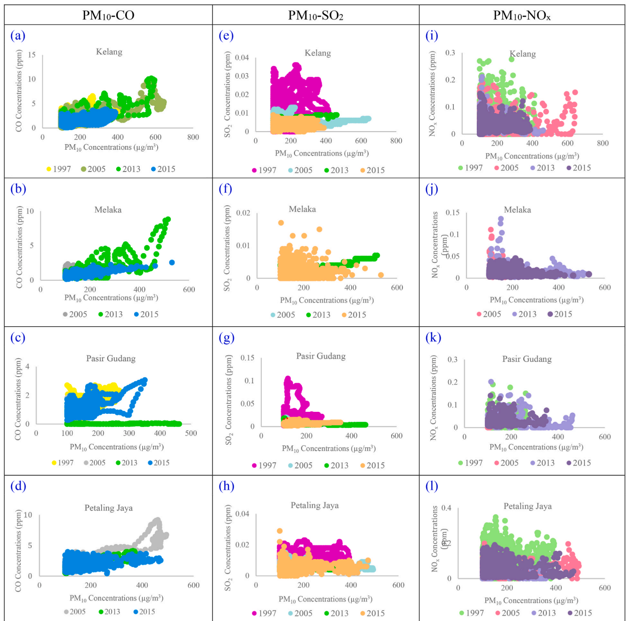
Fig. 5. Scatter plot of PM 10 -CO (a–d), PM 10 -SO 2 (e–h) and PM 10 -NO x (i–l) during the haze episodes.
