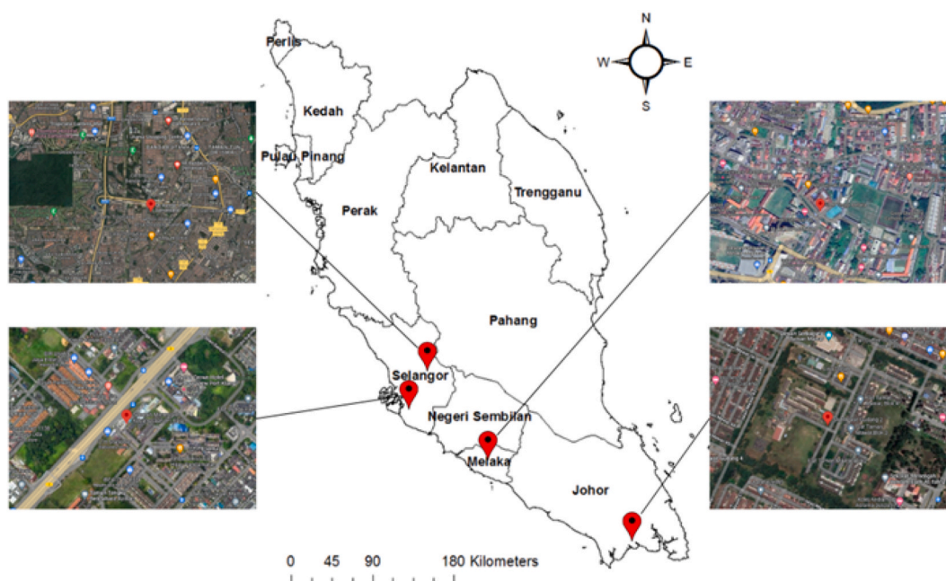
Fig. 1. The locations of the study.
