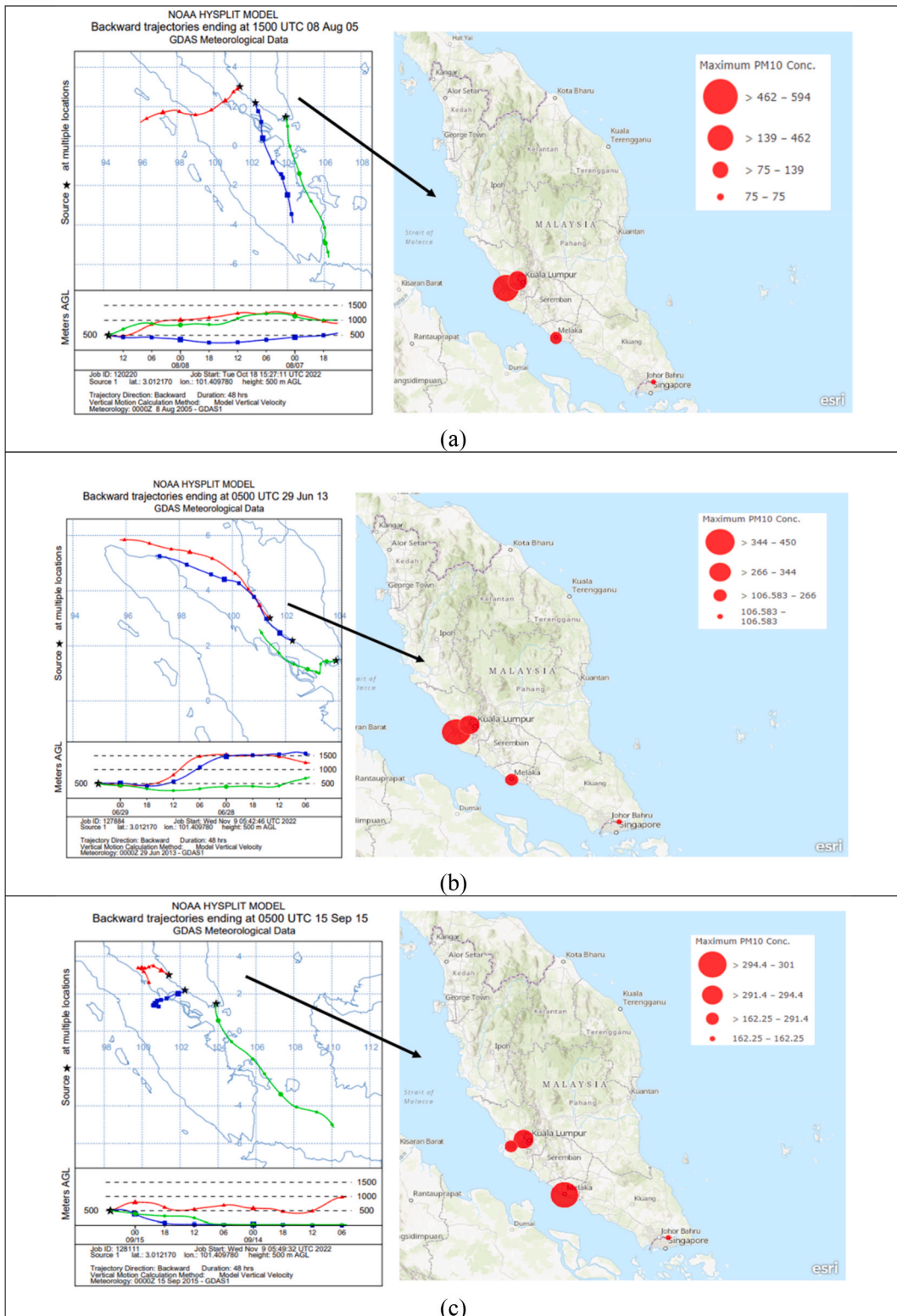
Fig. 4. The backward trajectories of wind and the spatial distribution of PM 10 concentration during haze event in (a) 2005; (b) 2013 and; (c) 2015.
