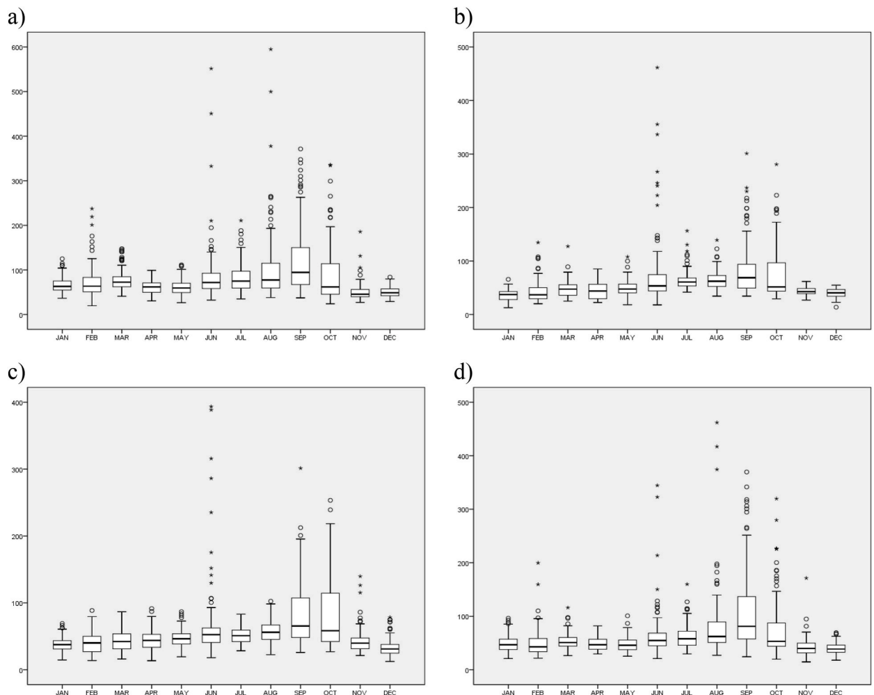
Fig. 3. Box plot distribution for PM 10 concentrations at a) Kelang, b) Melaka, c) Pasir Gudang and d) Petaling Jaya.
