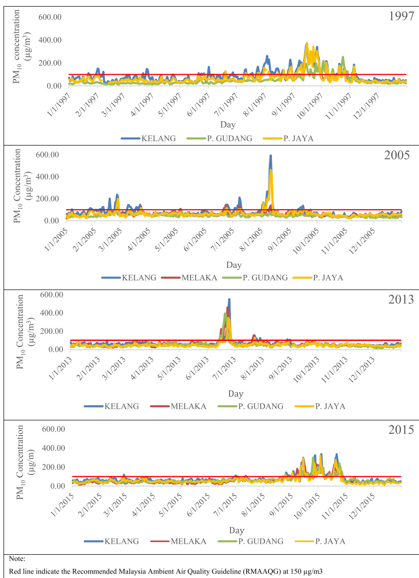
Fig. 2. Daily time-series plot for Kelang, Melaka, Pasir Gudang and Petaling Jaya.
