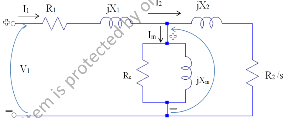
Figure 2.2: Induction machine per phase equivalent circuit (M.Thirugnanasambandamoorthy et.al, 2011)
