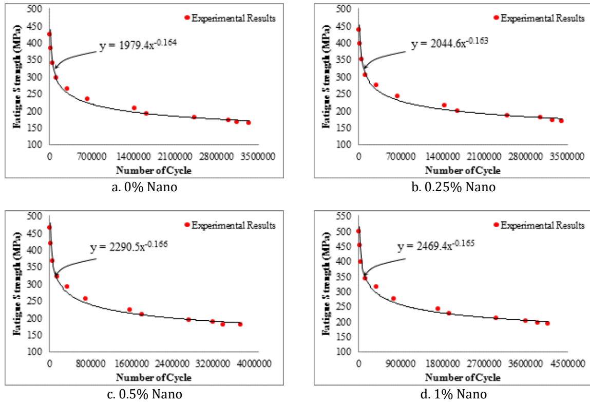
Figure 16. Curve fitting for experimental fatigue results with nanoparticle coating and laser treatment.
