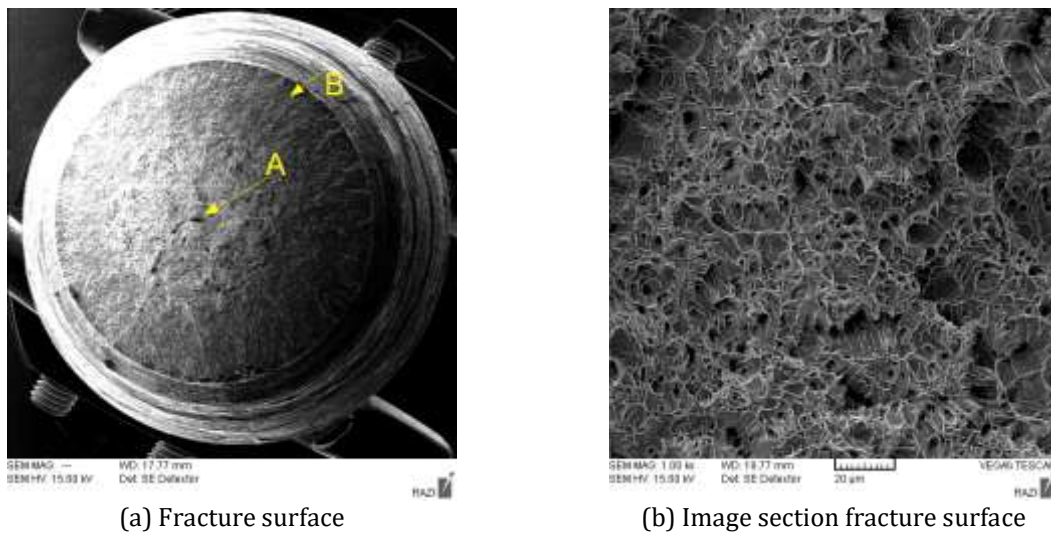
Figure 5. SEM view of the fracture surface (0% nano) sample.
