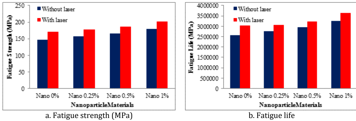
Figure 14. Fatigue strength and life for steel samples with nanoparticle and laser treatment effect.
