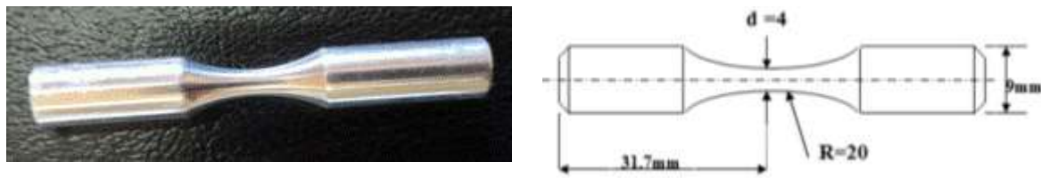
Figure 1. (a) Fatigue manufacturing sample; (b) Dimensions of fatigue test specimen.
