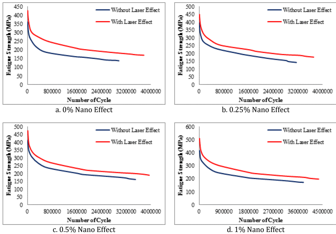
Figure 12. Results for laser treatment and nano effect on the fatigue characterizations for materials.
