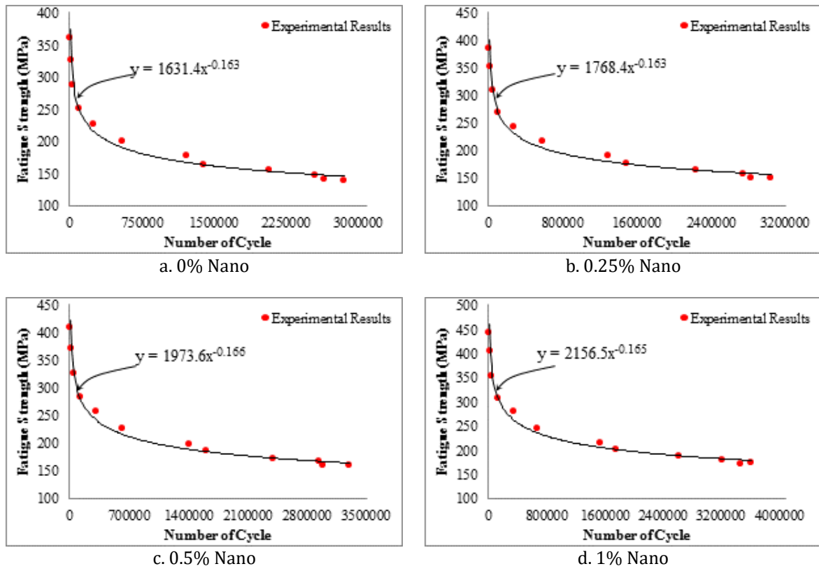
Figure 15. Curve fitting for experimental fatigue results with nanoparticle effect, without laser treatment.
