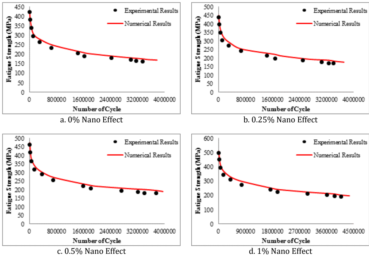
Figure 11. Numerical and experimental fatigue results comparison for steel materials with nanomaterial and laser treatment effect.
