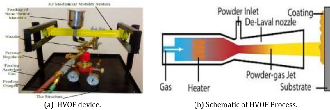
Figure 2. HVOF device and process.
