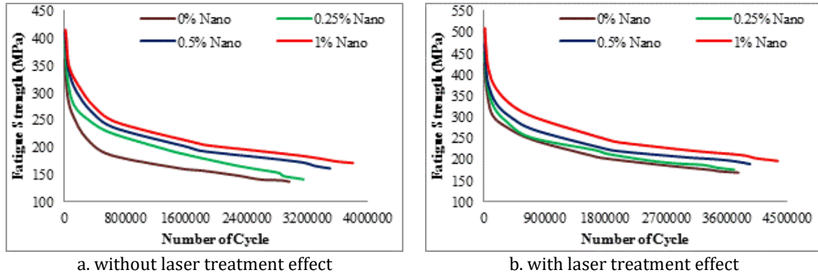
Figure 13. Fatigue characterizes material with and without laser treatment and nano effects.
