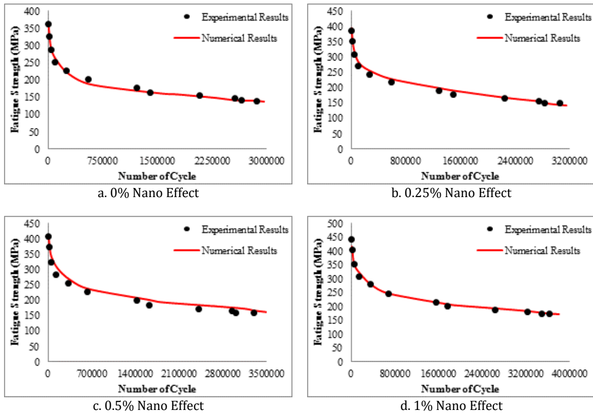
Figure 10. Numerical and experimental fatigue results comparison for steel materials with nanomaterial.
