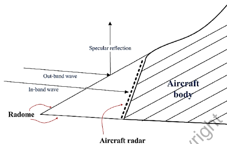
Figure 2.2: Application of frequency-selective surfaces as radome covers in the aircraft technology for reducing the antenna RCS (Munk, 2000).
