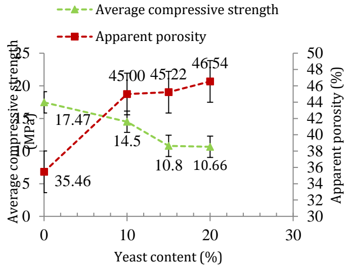
Figure 5 Relationship between average compressive strength and apparent porosity as functions of yeast content
