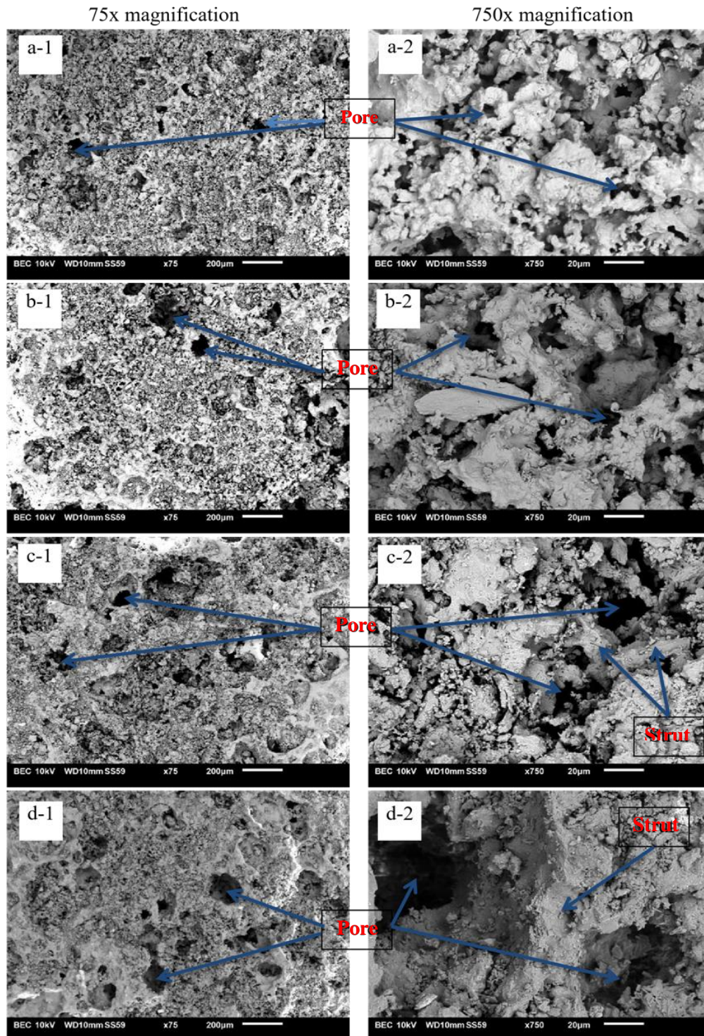
Figure 3 Macrostructure of sintered porous ceramic: (a) 0 wt.%, (b) 10 wt.%, (c) 15 wt.% and (d) 20 wt.% at 75x and 750x magnification by using scanning electron microscope (SEM)
