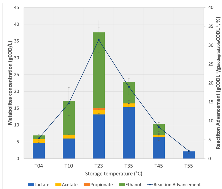
Fig. 2. Cumulated final metabolites concentration of stored food waste (SFW) according to the storage temperature and extent of the reaction advancement.
