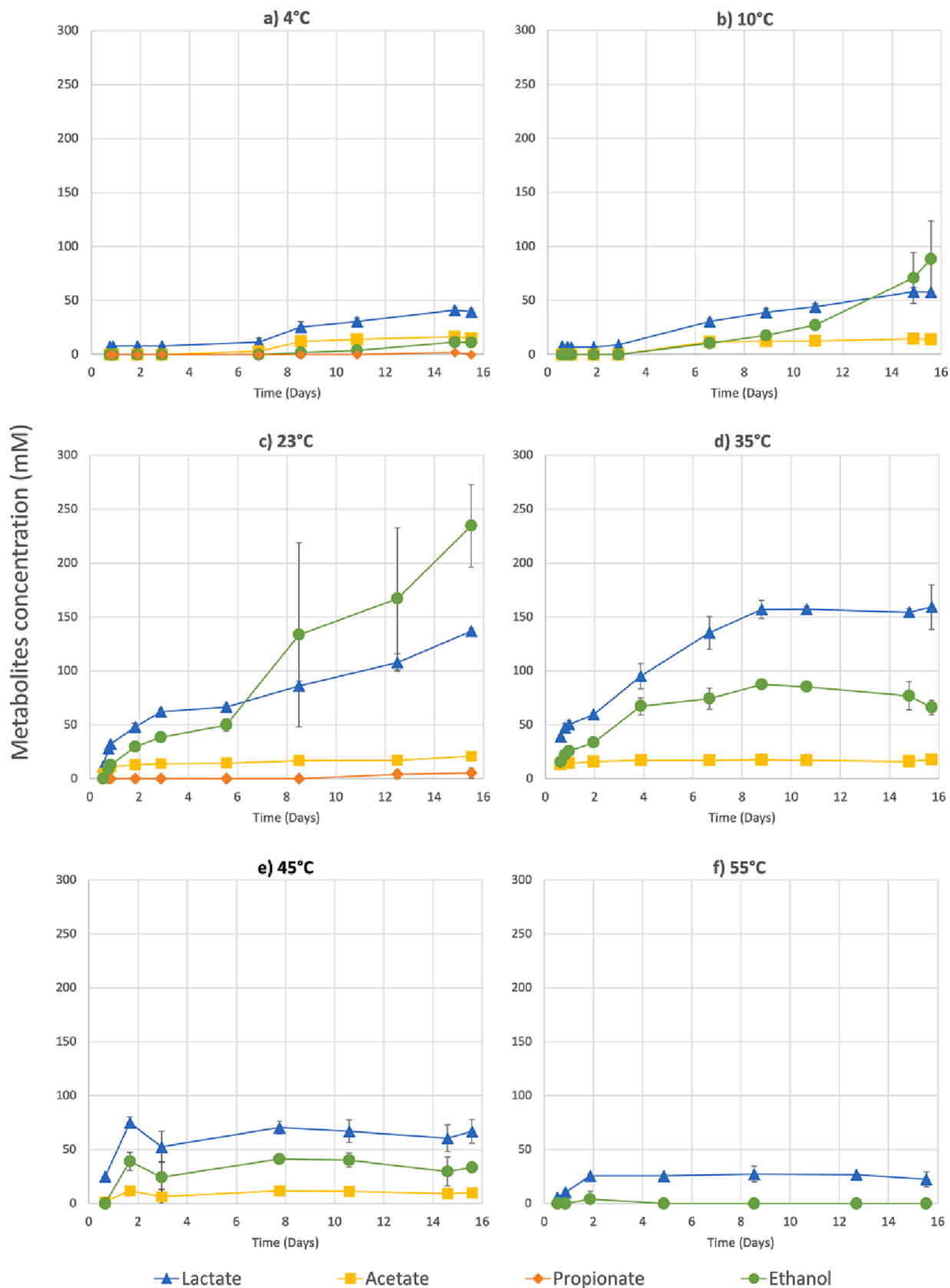
Fig. 1. Accumulation of metabolites during 15 days of storage at temperature of a) 4 °C, b) 10 °C, c) 23 °C, d) 35 °C, e) 45 °C and f) 55 °C. Metabolites not detected or below quantification limit were not plotted.
