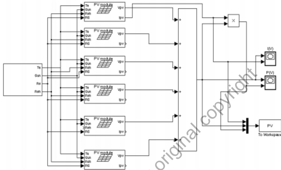
Figure 2.2: Photovoltaic cell array model Source: Salmi et al. (2012)
