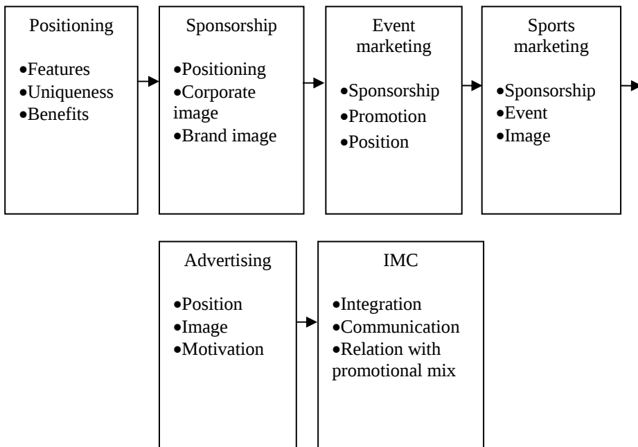
Figure 1: PSESAT Model
