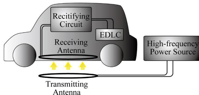
Figure 2.3 : The WPT for Electric Vehicles (Imura, Uchida, & Hori, 2009)
