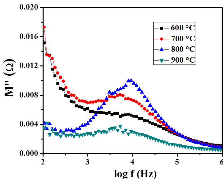
Figure 9. Patterns at various temperatures from 600 °C to 900 °C of frequency dependent imaginary part of electric modulus for cobalt ferrite nanoparticles
