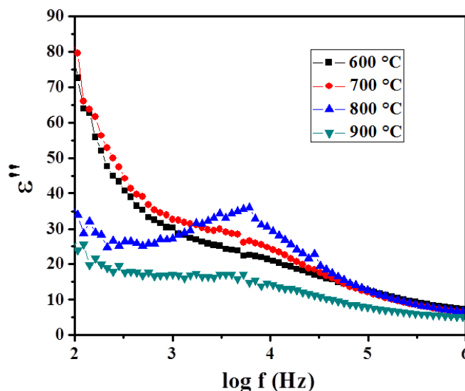
Figure 4. Complex dielectric constant patterns of cobalt ferrite nanoparticles at various temperatures from 600 °C to 900 °C with frequency dependency
