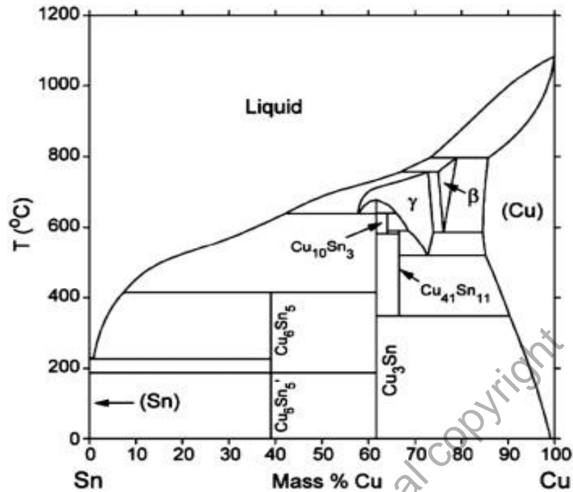
Figure 2.2: Phase diagram of Sn-Cu system (Prabhu, 2011)
