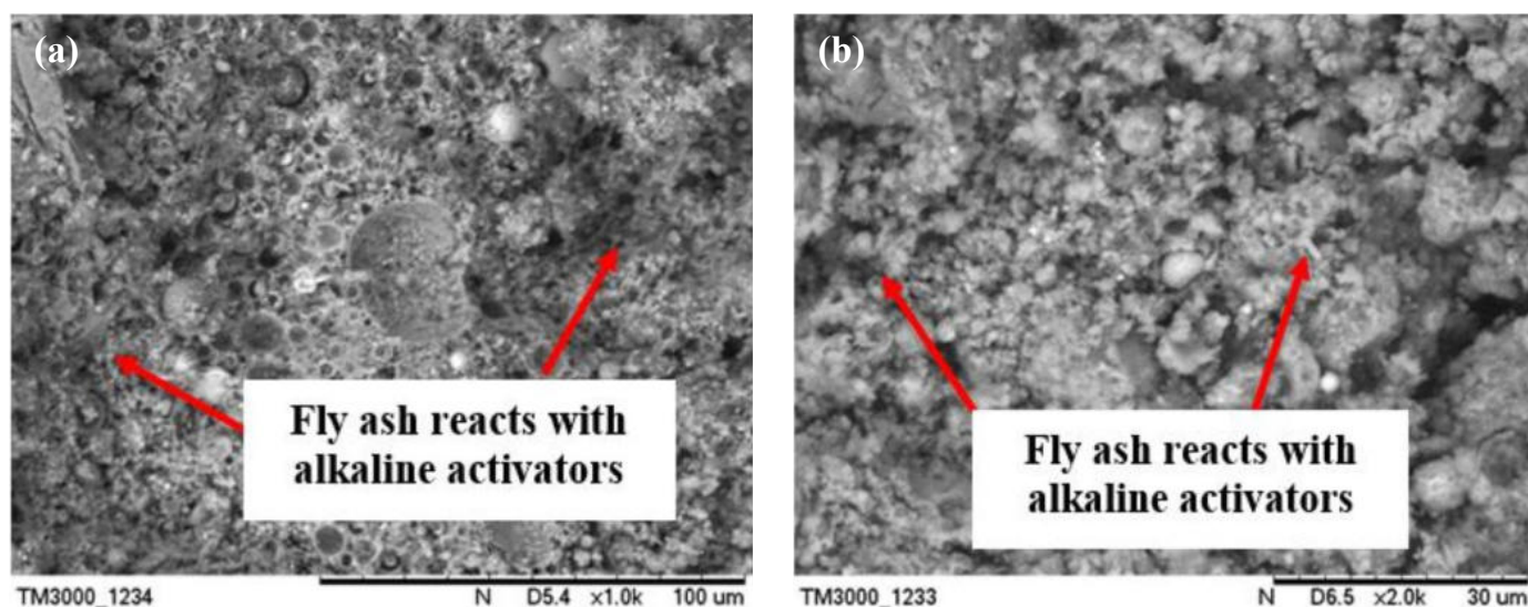
Fig. 5. SEM micrographs of curing geopolymer paste based fly ash after 28 days (a) \times 1000 and (b) \times 2000
