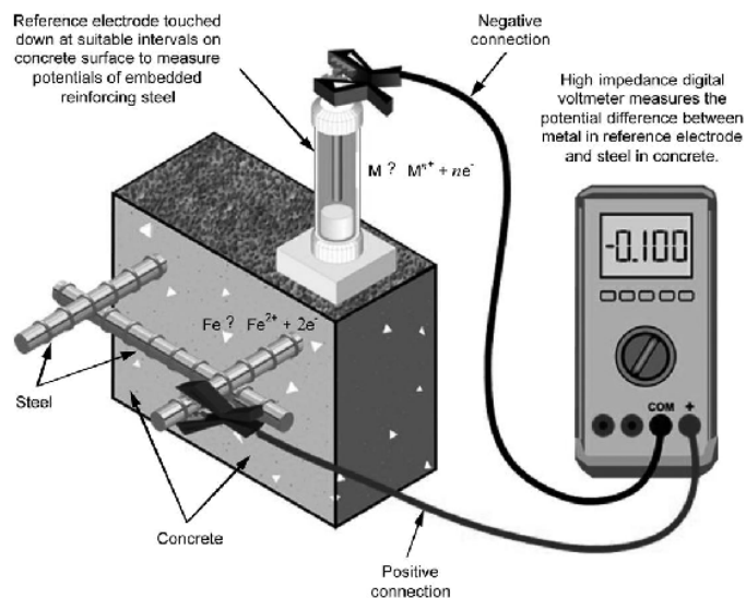
Fig. 1. Open Circuit Potential setup
