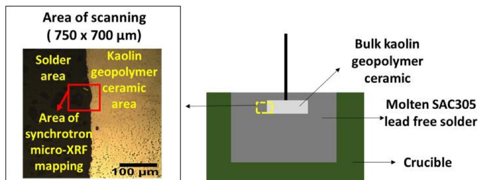
Fig. 2. Schematic diagram for the experimental setup dipping of bulk kaolin geopolymer ceramic in SAC305 lead free solder.
